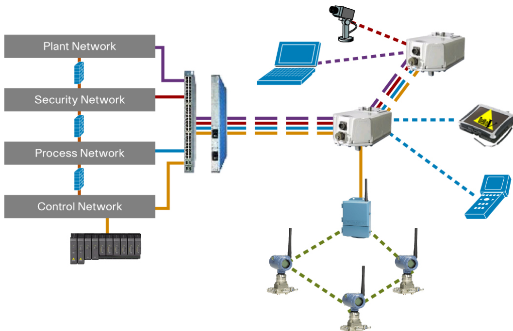
Figure 1. The Cisco Sensor Network Architecture
